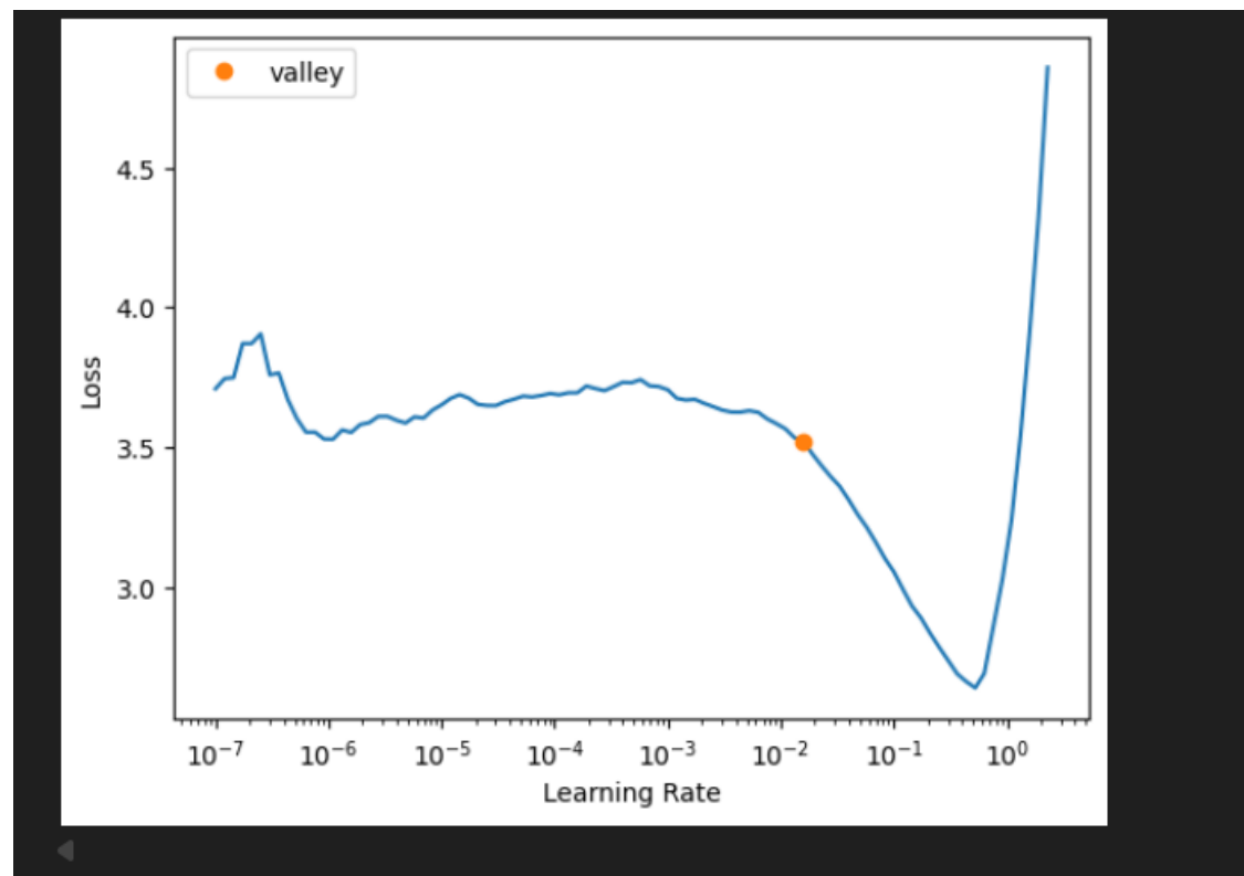
Figure 4: Learning rate graph
